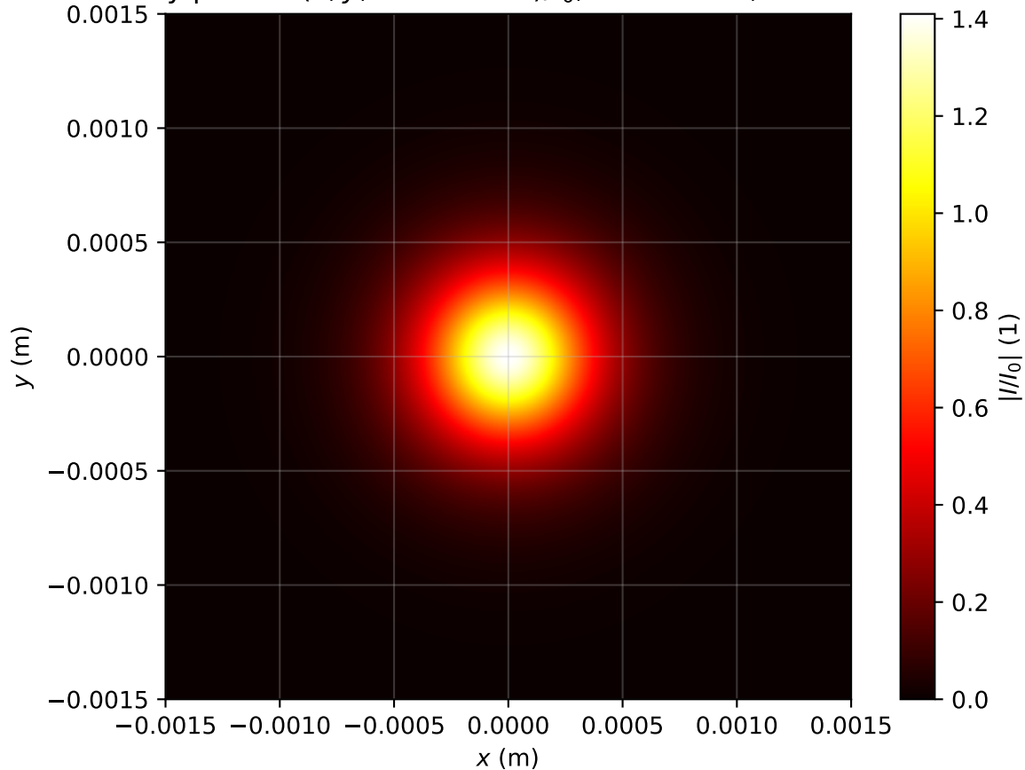
Intensity profile I(x, y, z = 3.981m)/I_0 , Pin=0.9Pcr, artificial time
